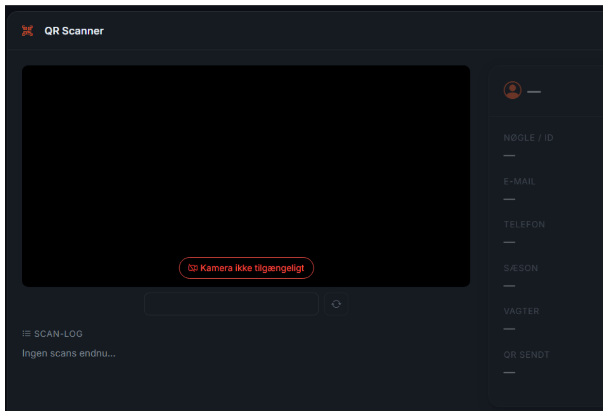
QR Scanner
